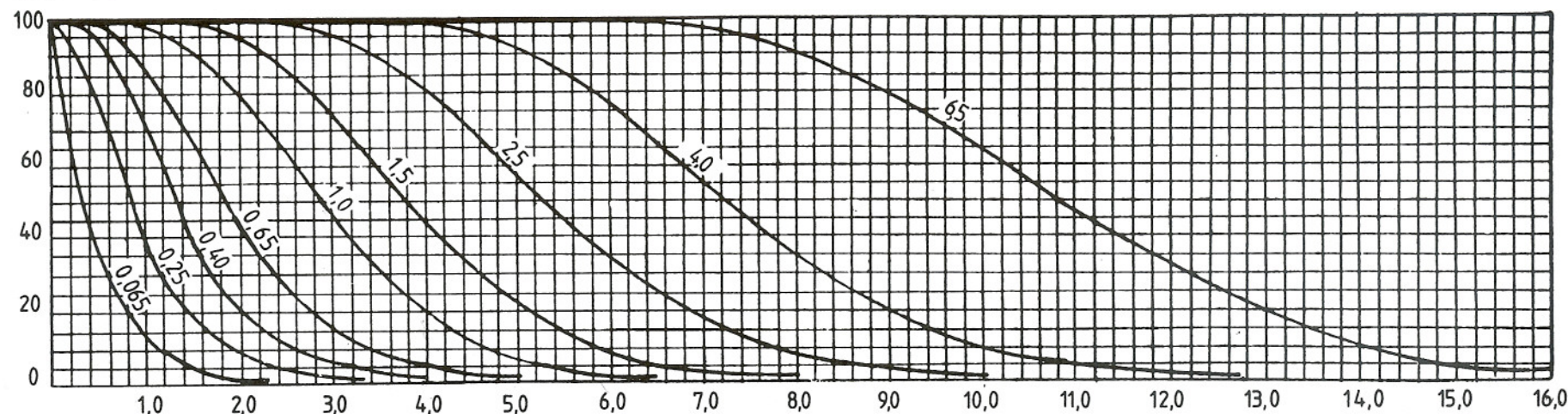
Chart L — Operating characteristic curves for single sampling plans (Curves for double and multiple sampling are matched as closely as practicable)
