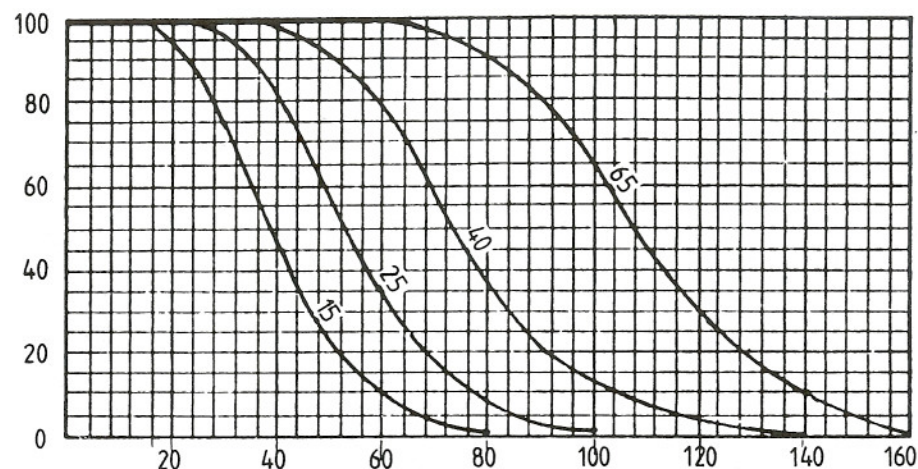
Chart F — Operating characteristic curves for single sampling plans (Curves for double and multiple sampling are matched as closely as practicable)
