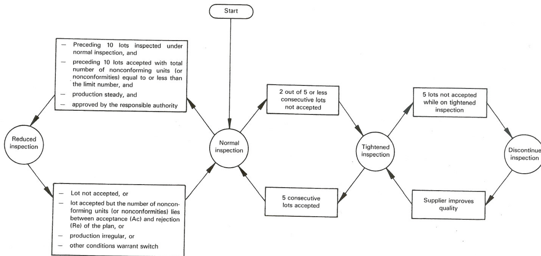
Figure 1 — Outline of the switching rules (see 9.3)
