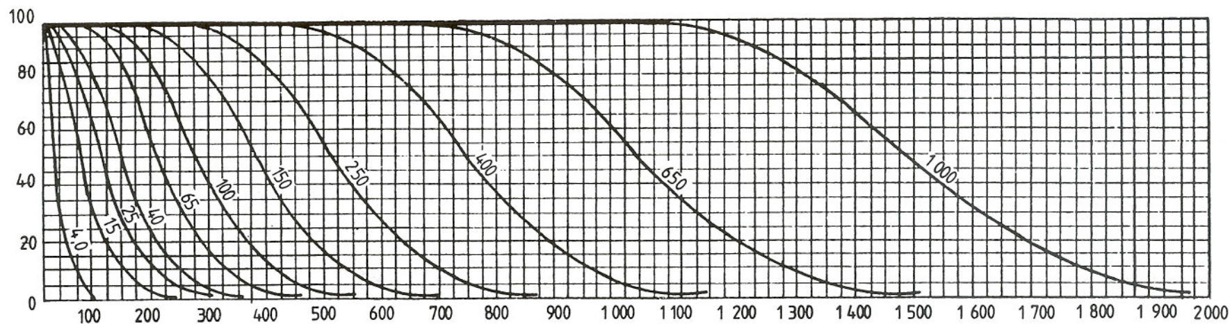
Chart B — Operating characteristic curves for single sampling plans (Curves for double and multiple sampling are matched as closely as practicable)
