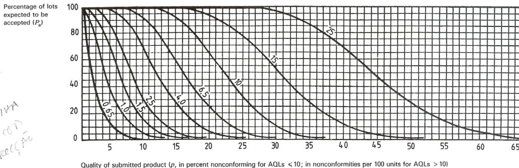
Chart H — Operating characteristic curves for single sampling plans (Curves for double and multiple sampling are matched as closely as practicable)
