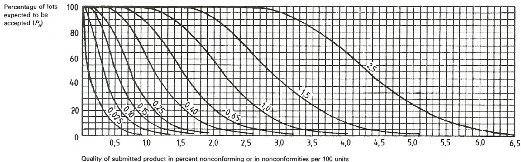
Chart N — Operating characteristic curves for single sampling plans (Curves for double and multiple sampling are matched as closely as practicable)
