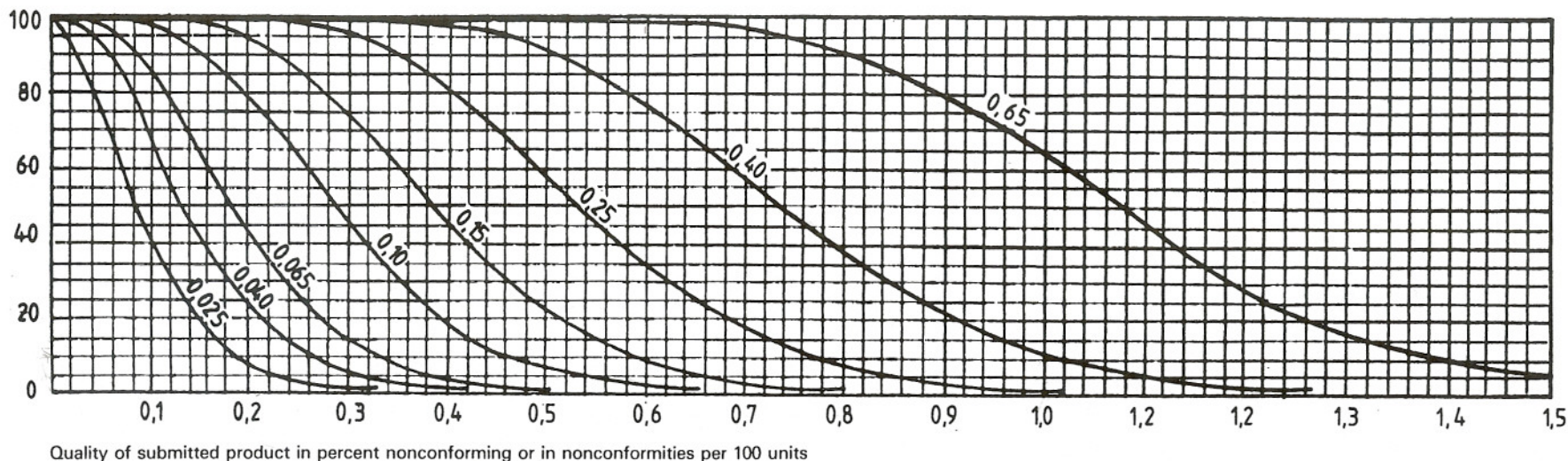
Chart R — Operating characteristic curves for single sampling plans (Curves for double and multiple sampling are matched as closely as practicable)
