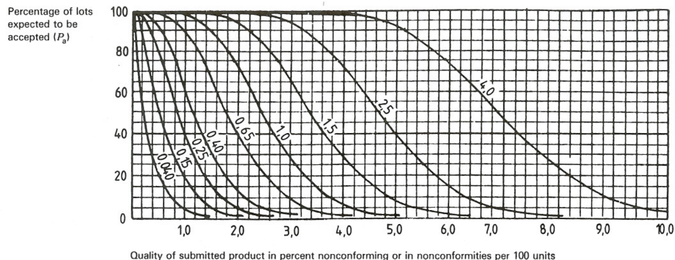
Chart M — Operating characteristic curves for single sampling plans (Curves for double and multiple sampling are matched as closely as practicable)
