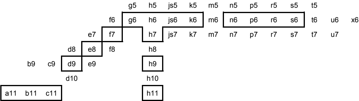
Figure 11 — Shafts
