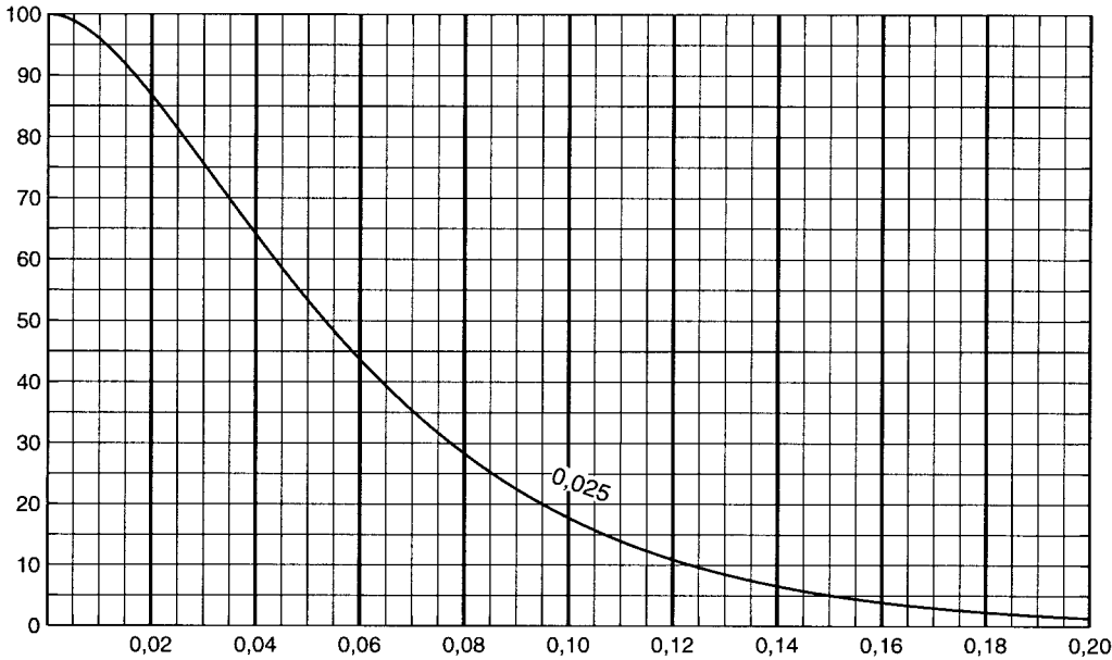
Chart S Operating characteristic curves for single sampling plan (Curves for double and multiple sampling are matched as closely as practicable)
