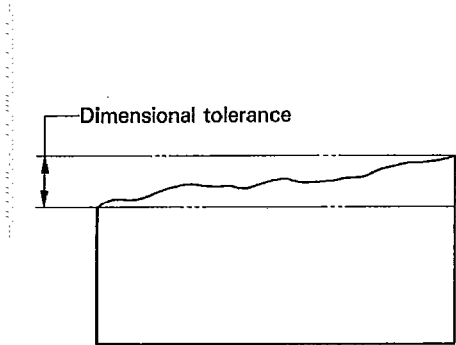
Figure B.3 — Parallelism deviation equal to the numerical value of the size tolerance
