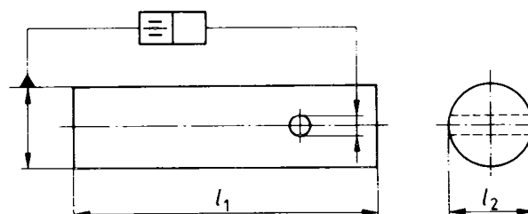
d) Datum: longer feature ( l_1 )
