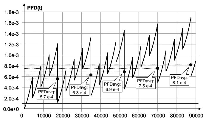
Figure B.22 – Example of complex testing pattern
