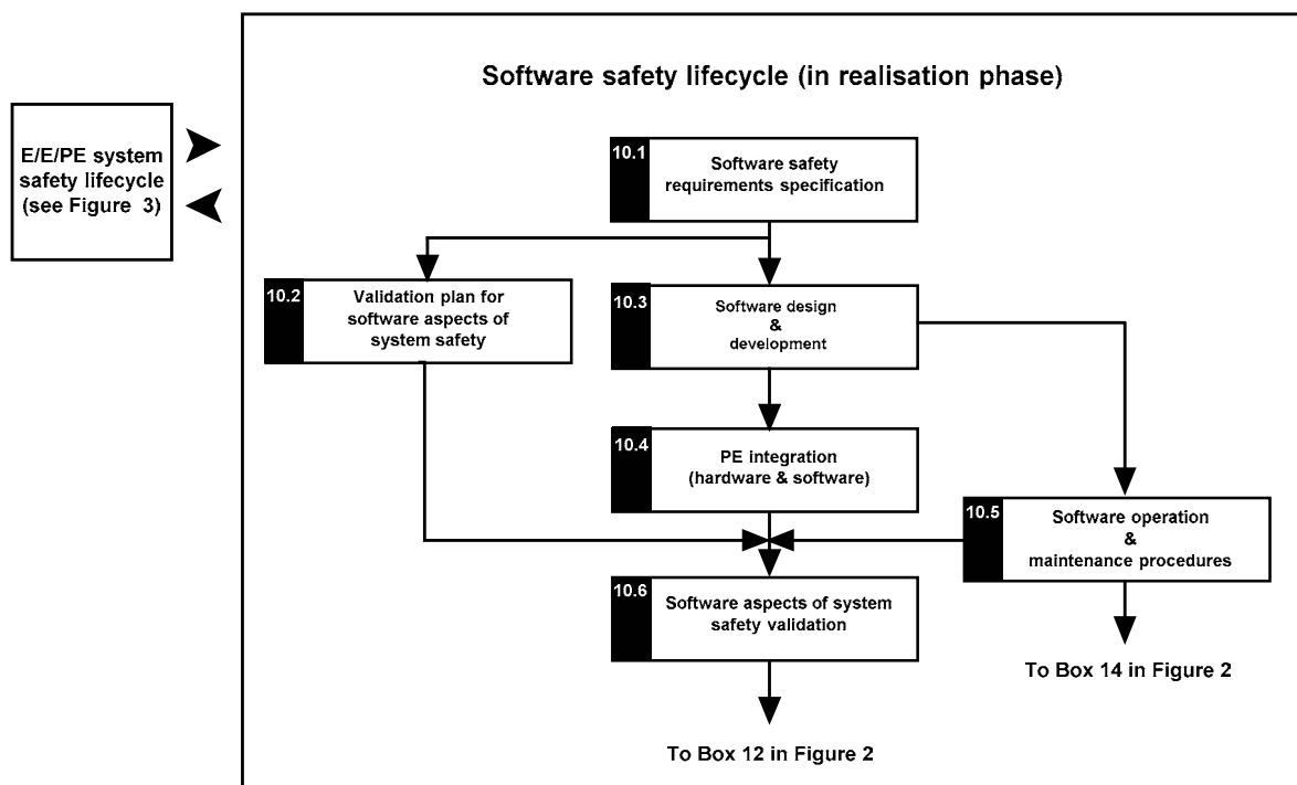
Figure 3 4 – Software safety lifecycle (in realisation phase) (42)
