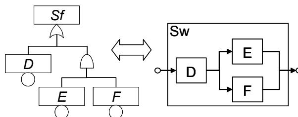
Figure B.18 – Equivalence fault tree / reliability block diagram
