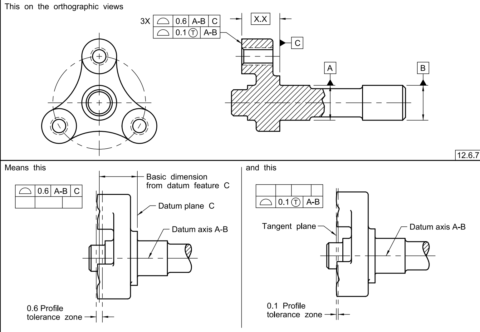
Figure 12-15 Surface Profile Tolerance Applied to a Tangent Plane
