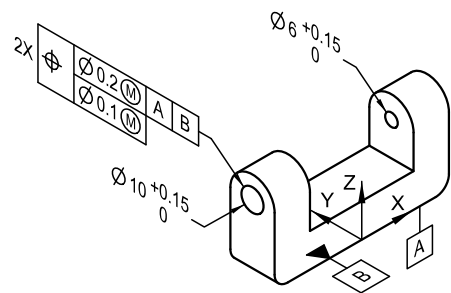
Figure 10-52 Positional Tolerancing for Multiple Features of More Than One Size
