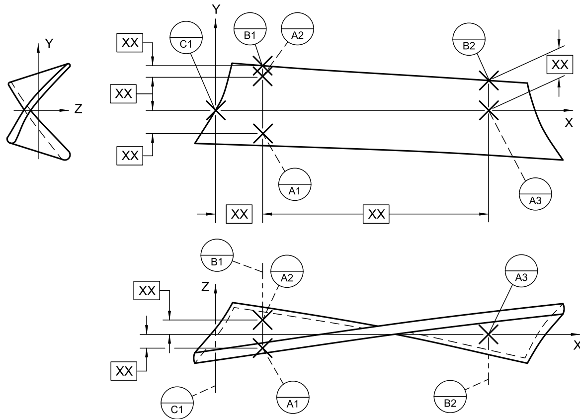
Figure 7-53 Datum Targets Used to Establish Datum Reference Frame for Complex Part
