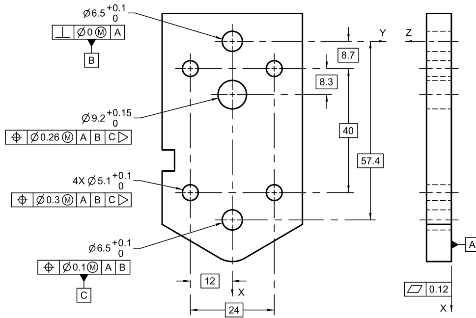
Figure 7-12 Development of a Datum Reference Frame With Translation Modifier
