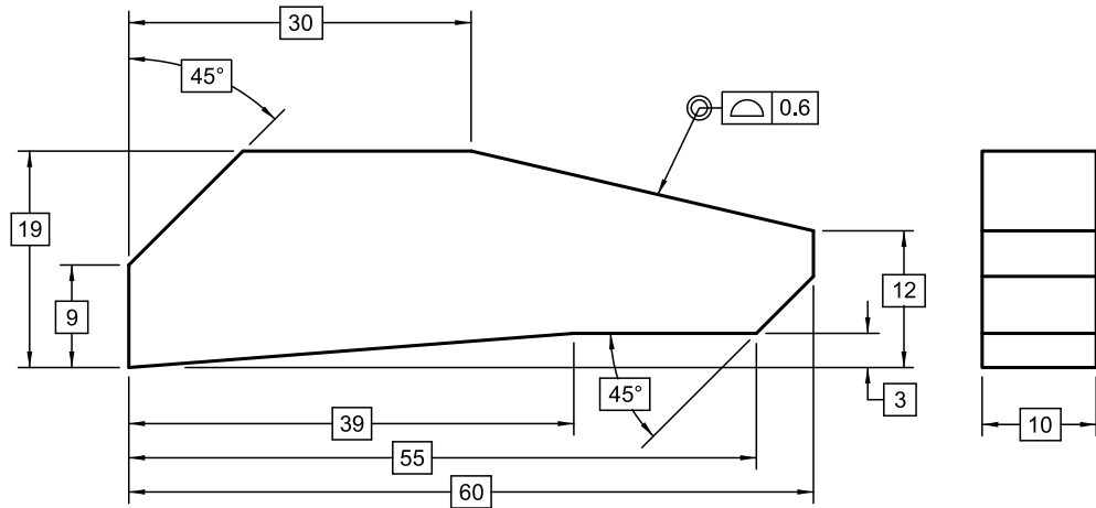
Figure 11-10 Specifying Profile of a Surface All Over
