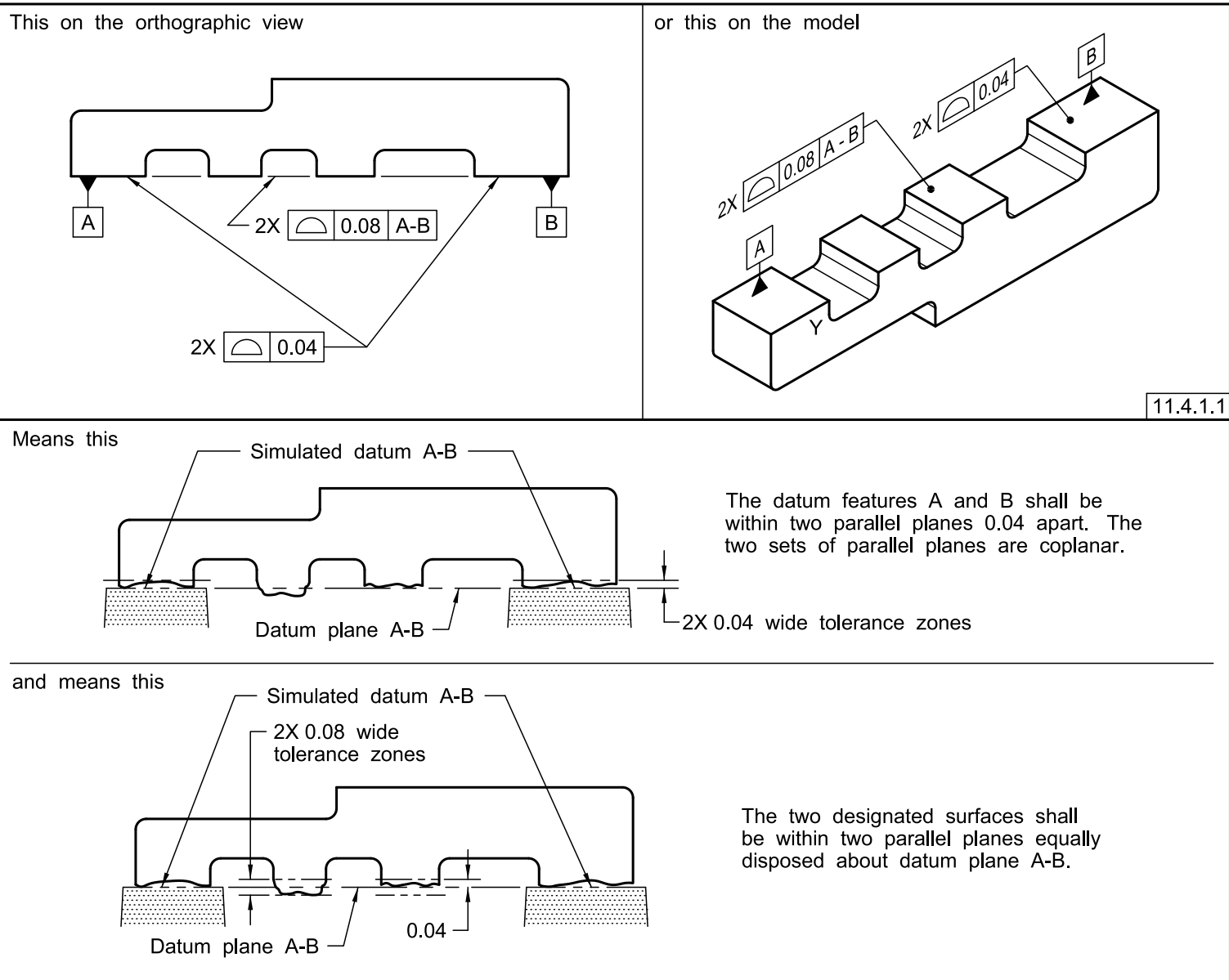
Figure 11-17 Specifying the Profile of a Surface for Coplanar Surfaces to a Datum Established by Two Surfaces
