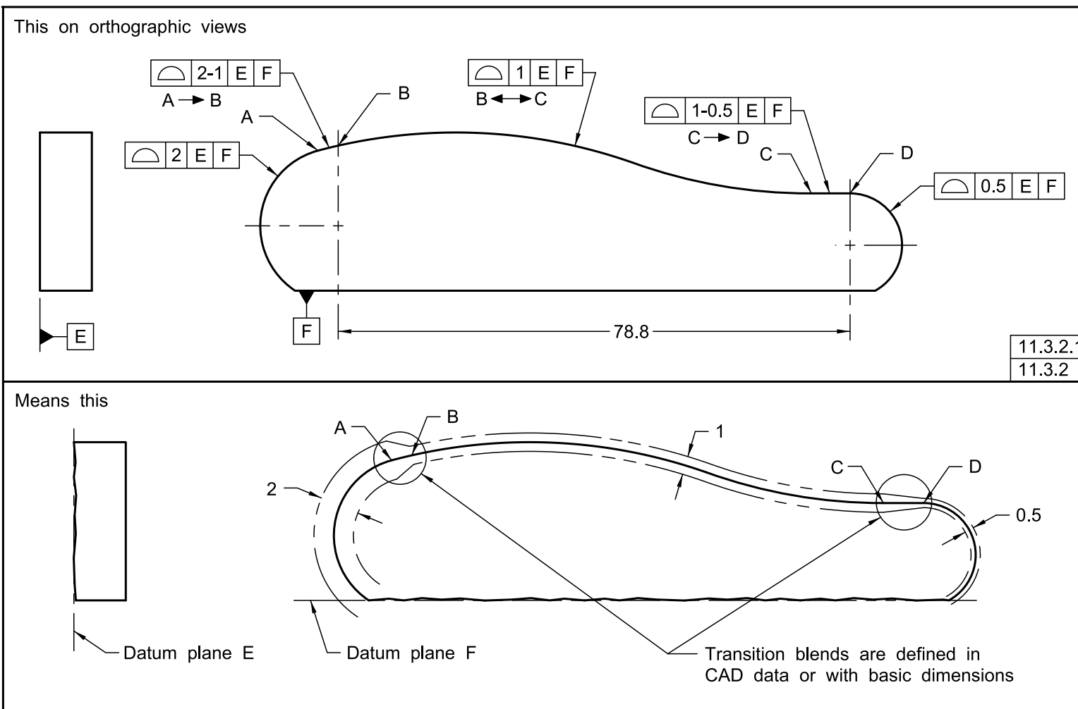
Figure 11-13 Nonuniform Profile Tolerance Zone With Zones to Smooth Transitions
