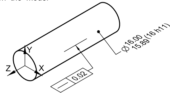
Figure 8-2 Specifying Straightness of Surface Elements
