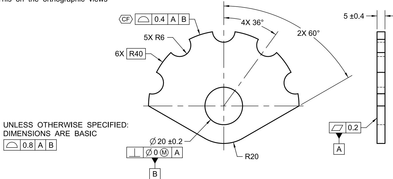
Figure 11-23 “Continuous Feature” Symbol Application in a Profile Tolerance
