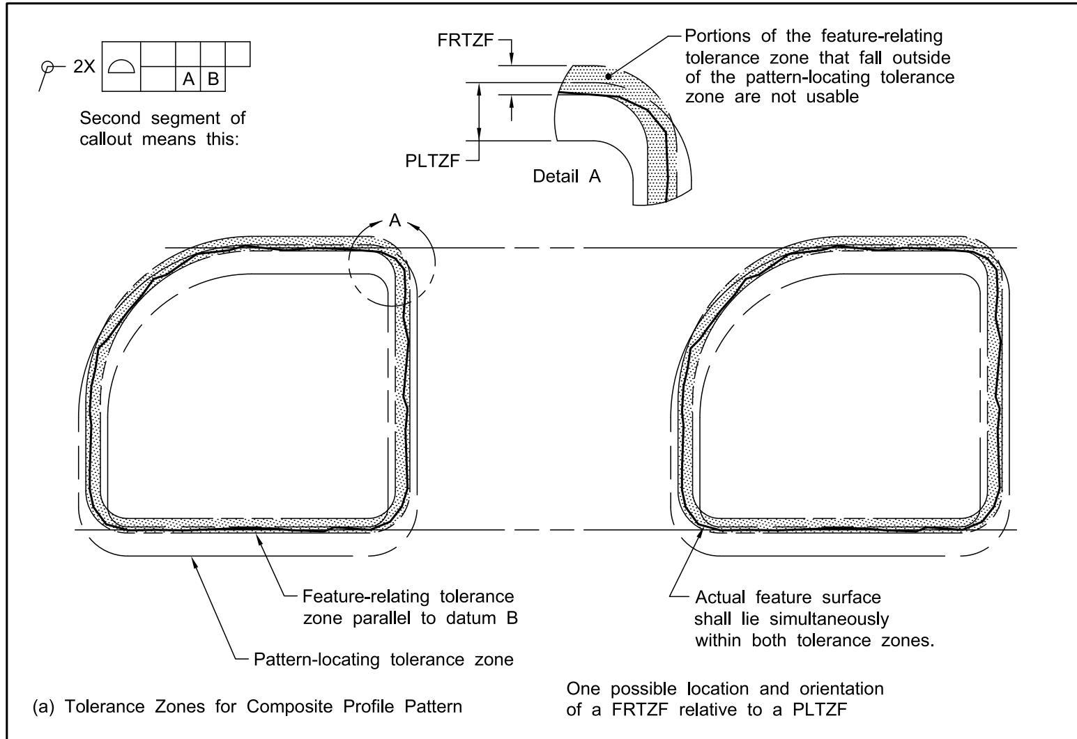
Figure 11-27 Pattern Located by Composite Profile Tolerancing — Repeated Primary and Secondary Datum Feature References (Cont'd)
