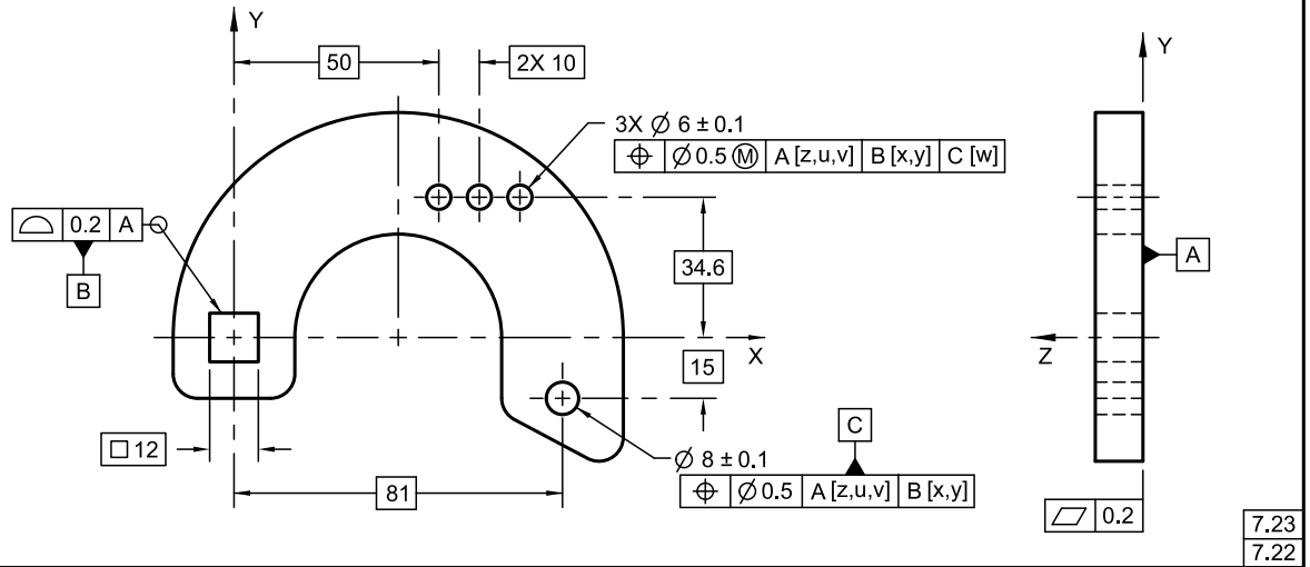
Figure 7-57 Customized Datum Reference Frame
