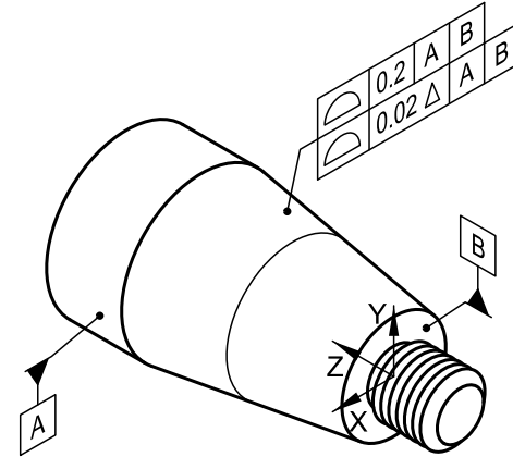
Figure 11-20 Profile Tolerancing of a Conical Feature, Datum Related
